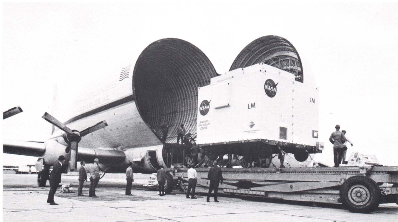
The separately packaged Lunar Module stages are placed aboard the Super Guppy aircraft for the flight to NASA Kennedy Space Center.
